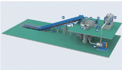
Low Consistency Pulping System
