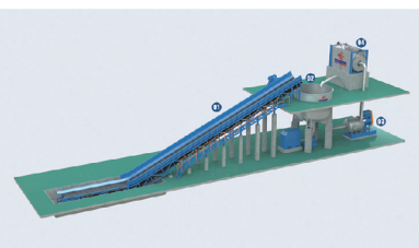
High Consistency Pulping System
