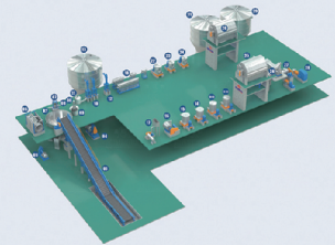
OCC Pulp Line System
