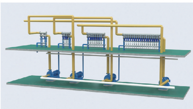
Low Consistency Cleaning System
