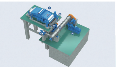
Twin-wire Press Hot Dispersing System
