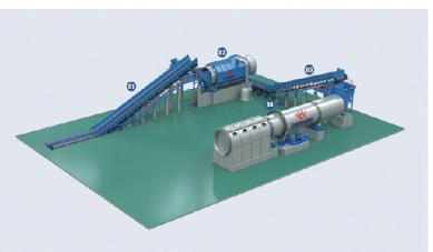
Bale Breaking & Drum Pulping System
